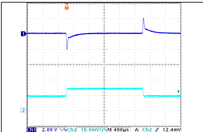
Figure 5: Output voltage response for QTC version of product to step-change in load current (50% -75% -50% of I out (max)); dI/dt = 0.6 A/µs). Load cap: 1 µF ceramic cap. Ch 1: V out , Ch 2: I out (1 A/div).
