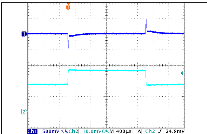
Figure 5: Output voltage response for QTC version of product to step-change in load current (50% -75% -50% of I out (max)); dI/dt = 0.6 A/µs. Load cap: 15 µF tantalum cap and 1 µF ceramic cap. Ch 1: V out , Ch 2: I out (2 A/div).
