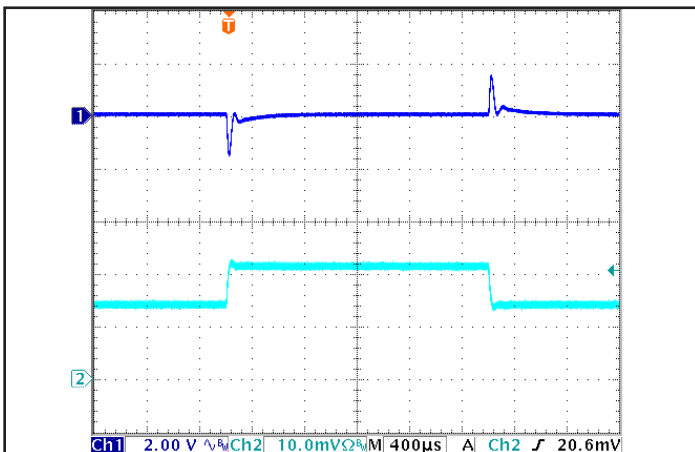
Figure 5: Output voltage response to step-change in load current for QTC version of product (50% -75% -50% of I out (max); dI/dt = 0.6 A/µs). Load cap: 1 µF ceramic cap. Ch 1: V out , Ch 2: I out (1 A/div).
