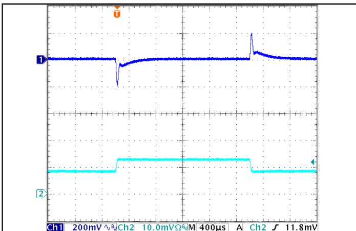
Figure 5: Output voltage response for QTC version of product to step-change in load current (50 % -75 % -50 % of I out (max)); dI/dt = 0.6 A/μs. Load cap: 15 μF tantalum cap and 1 μF ceramic cap. Ch 1: V out , Ch 2: I out (10 A/div).
