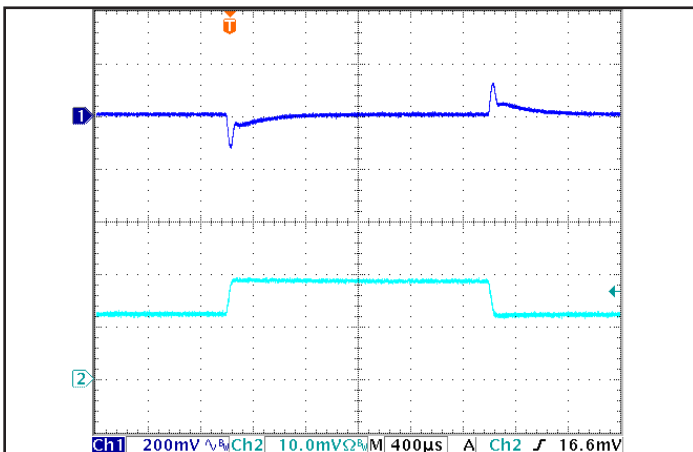
Figure 5: Output voltage response for QTC version of product to step-change in load current (50 % -75 % -50 % of I_{out(max)} ); dI/dt = 0.6 A/\mu s . Load cap: 15 \mu F tantalum cap and 1 \mu F ceramic cap. Ch 1: V out , Ch 2: I_{out} (10 A/div)
