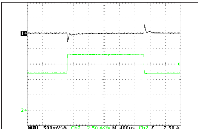
Figure 5: Output voltage response for QTC version of product to step-change in load current (50% -75% -50% of Iout(max)); dI/dt = 0.6 A/μs. Load cap: 15 μF tantalum cap and 1 μF ceramic cap. Ch 1: Vout, Ch 2: Iout.
